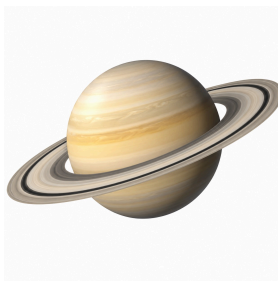
Saturn
